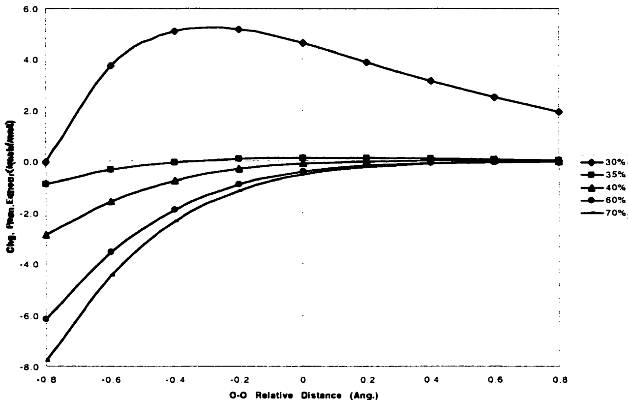
Fig. (2.2) Charge penetration error in kcal mol -1 as a function of oxygen-oxygen distance in the water dimer, and as a function of r_{\min} (separate curves). r_{\max} is 300% of the Van der Waals radius of each atom.
