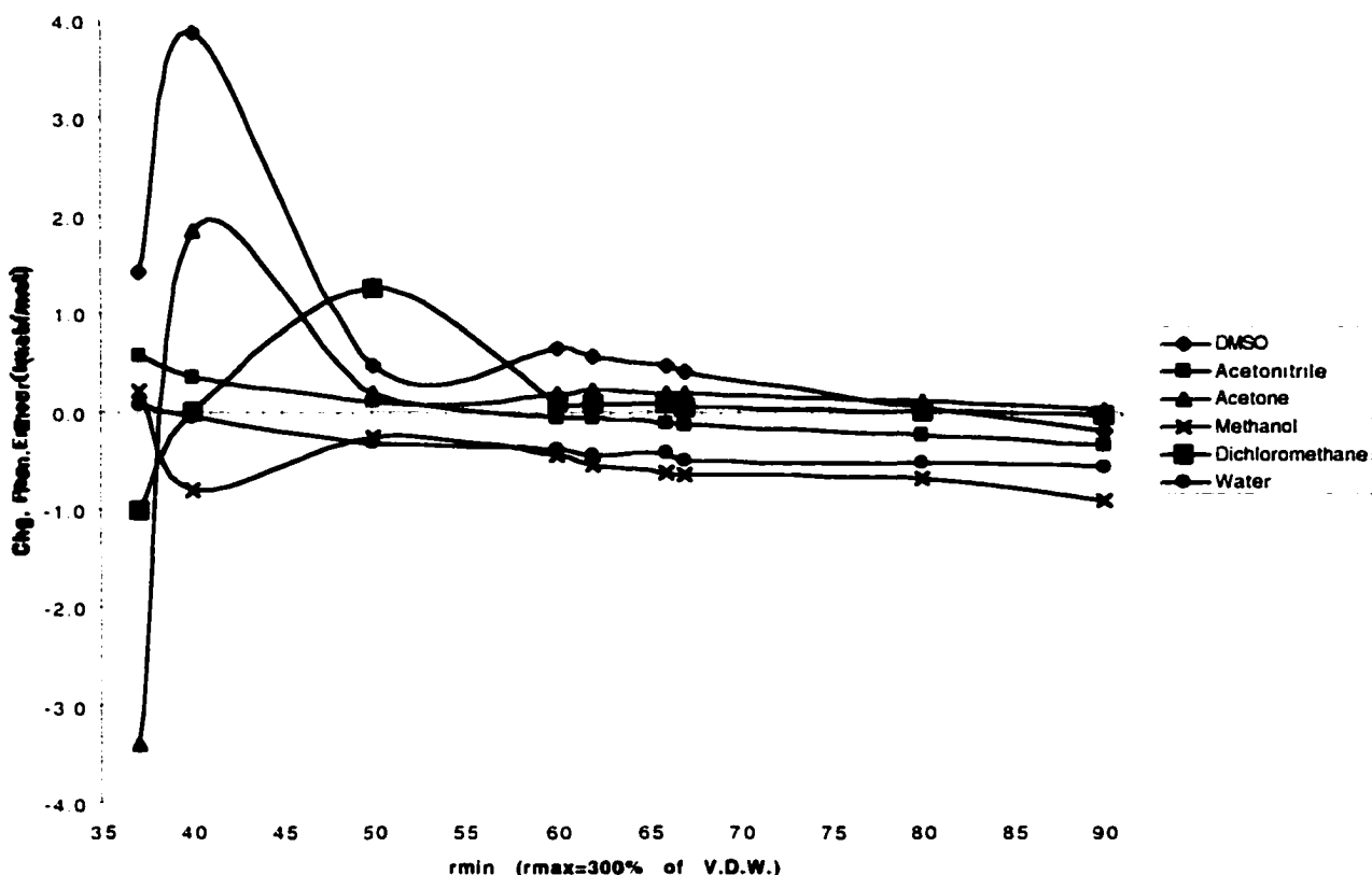
Fig. (2.3) Charge penetration error in kcal mol -1 for six homomolecular dimers at their equilibrium geometries, as described in the text. The charge penetration error is given as a function of r_{\min} . r_{\max} = 300\% of the Van der Waals radius on each atom.
